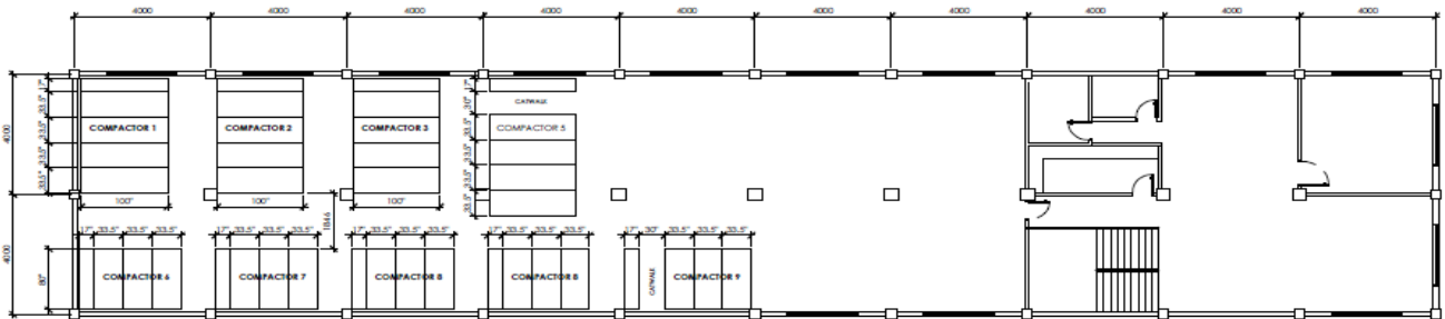
COMPACTOR LAYOUT
